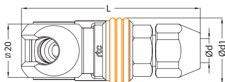
Socket / Kupplung
