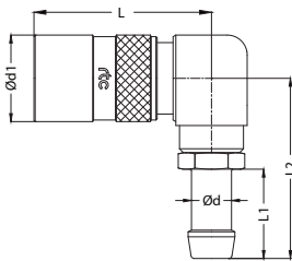
Socket / Kupplung
