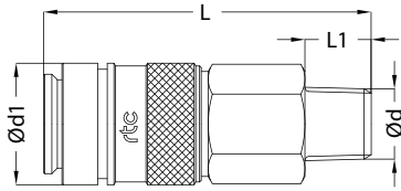
Sockets / Kupplungen
