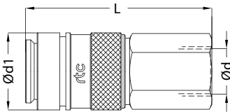
Sockets / Kupplungen
